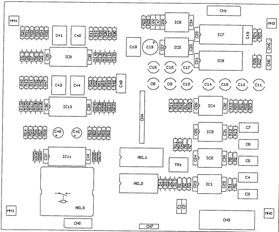
analog board mod. 1
