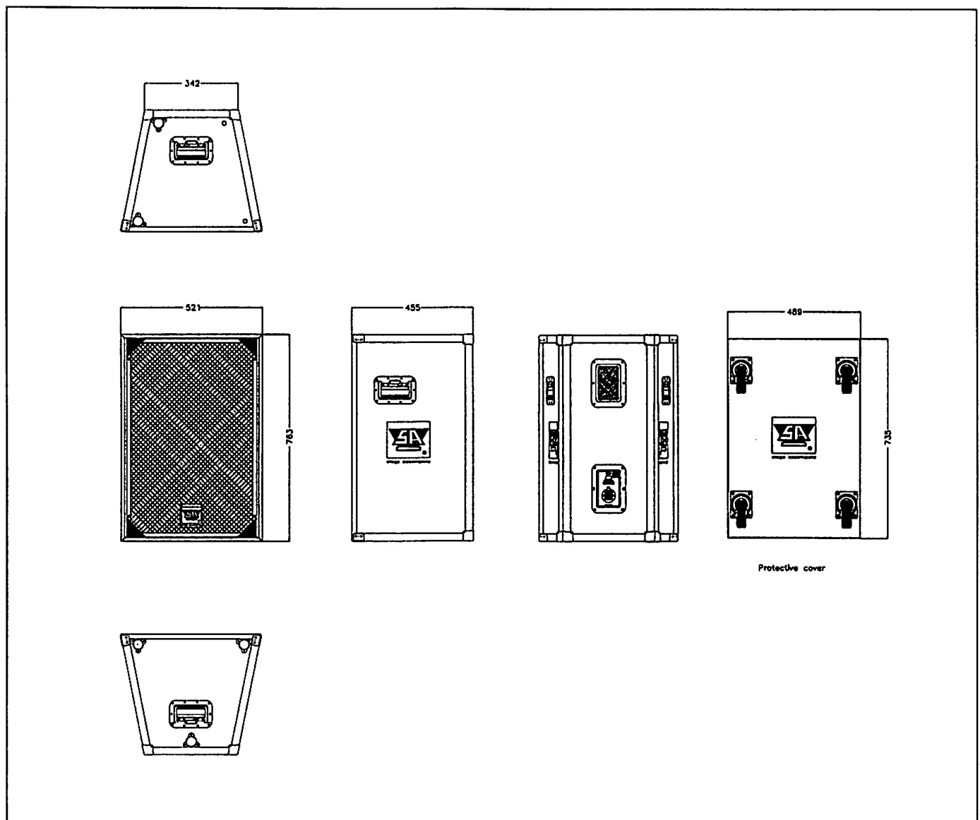
Physical dimensions of the SA 4827; flightcased version. The protective cover/dolly for transportation is shown at the right side.
