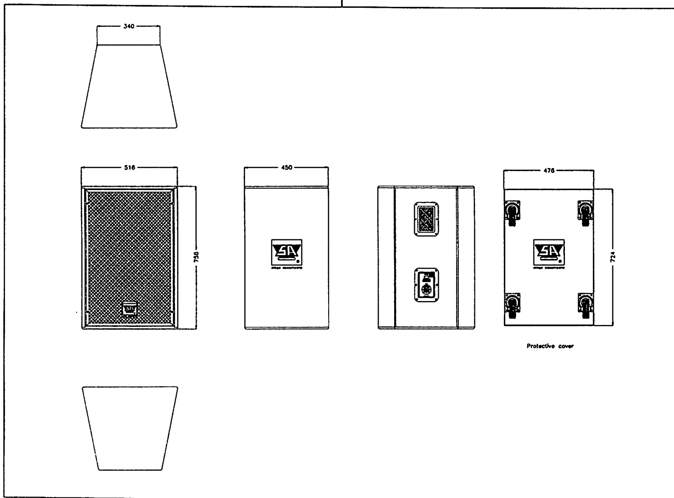
Physical dimensions of the SA 4827; normal version. The protective cover/dolly for transportation is shown at the right side.
